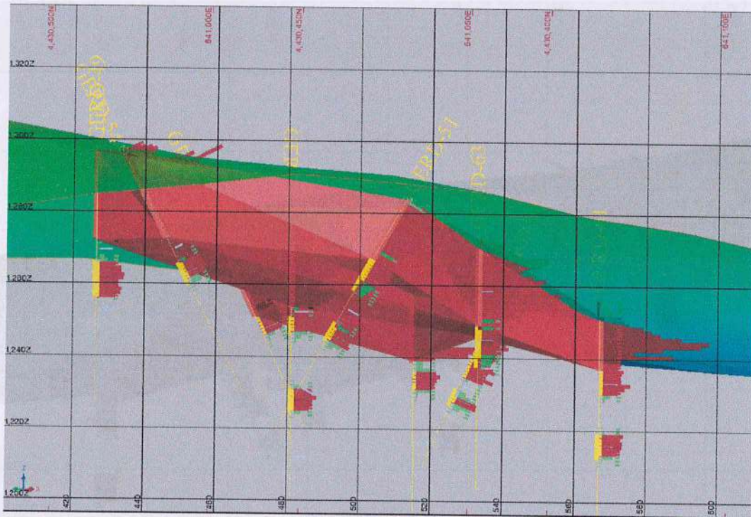
Figure 46. Wireframe B2 in section (location of black dashed section line is given in figure before; dashed black line).
