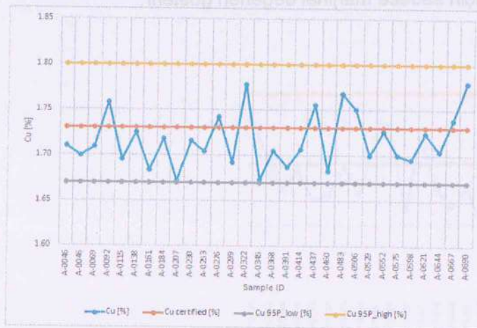
Figure 31. Assay results for CRM OREAS 623 for Cu.
