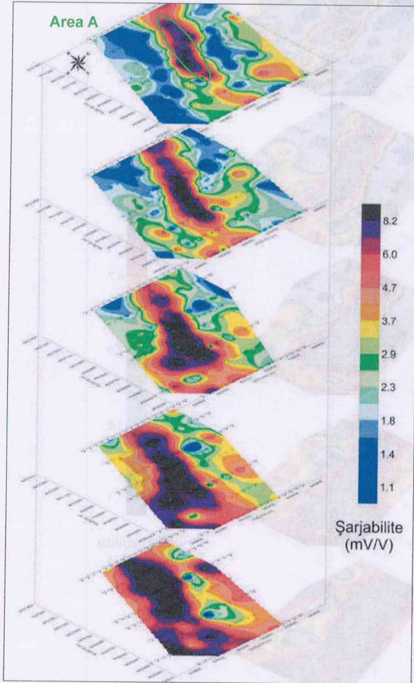
Figure 16. Stacked maps of chargeability.
