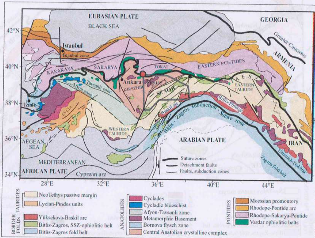
Figure 13. Tectonic map of western Tethys showing main tectonic units and mineral deposits. Simplified and modified from Stampfli et al. (1998), Stampfli (2001), Jolivet et al. (1994), and Kaymakçi and Kuscu (2007). Abbreviations: IAESZ = Izmir- Ankara-Erzincan suture zone, SEAOB = Southeastern Anatolian orogenic belt, SSZ = Suprasubduction zone (Source: Ilkay Kuscu et al., 2013); location of licence area (red point).
